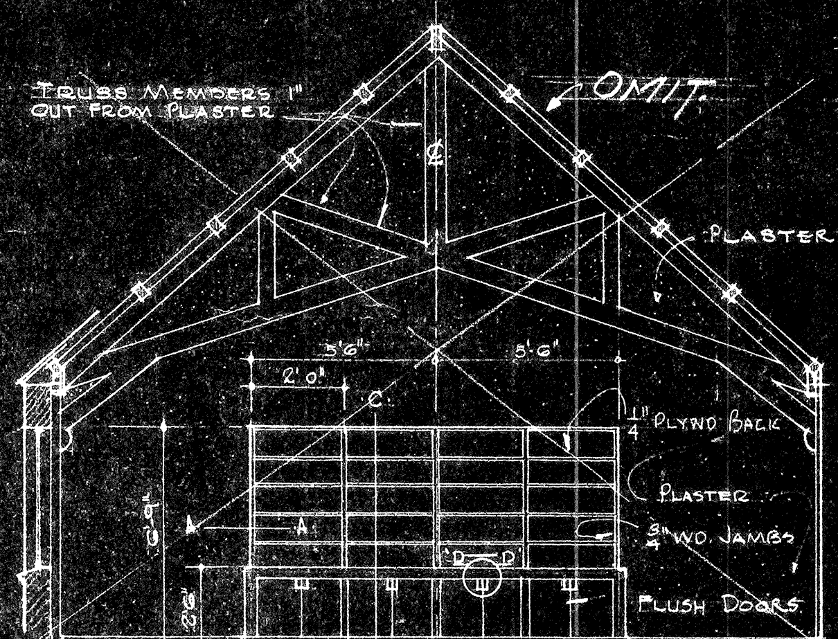
ELEVATION EAST END SCALE 1/4" = 1'-0"
