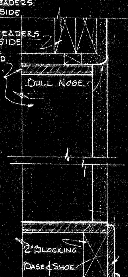
SECTION D-D SCALE 3/4" = 1'-0"
